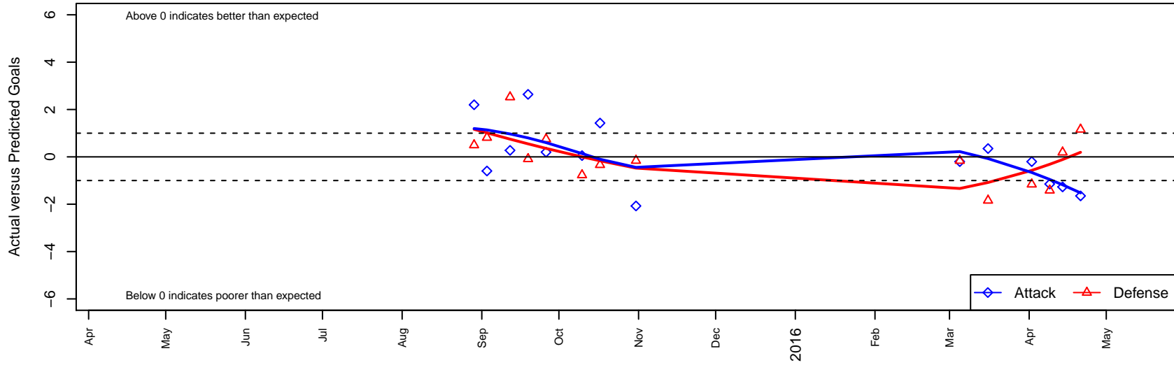
Idaho Torrent Valor G00 Dots are actual minus expected GF (blue circles) and GA (red triangles). Blue line is smoothed change in attack strength. Red is smoothed change in defense strength.
